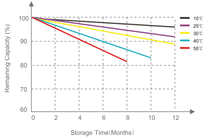
SELF DISCHARGE VS. TEMPERATURE
