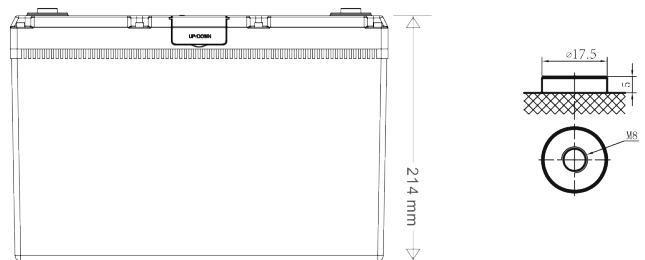
BATTERY DIMENSIONS
