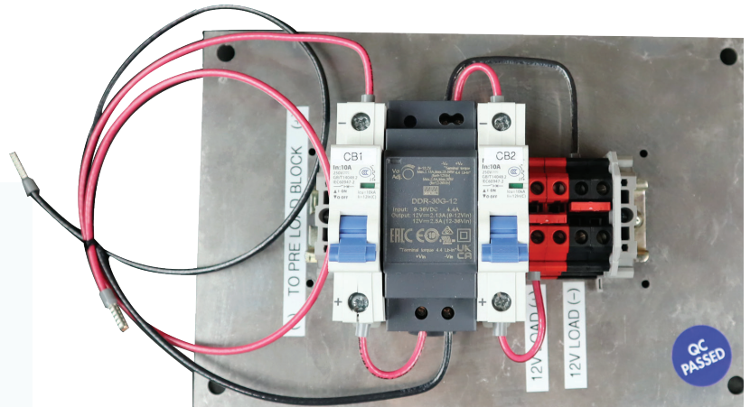
PRE Converter Accessory Control Panel
