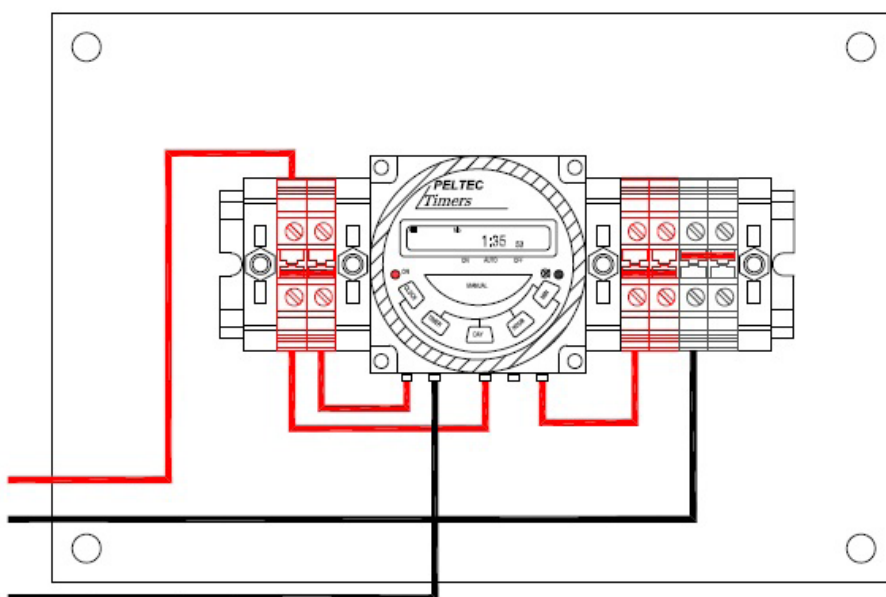
PRE Timer Accessory Panel
