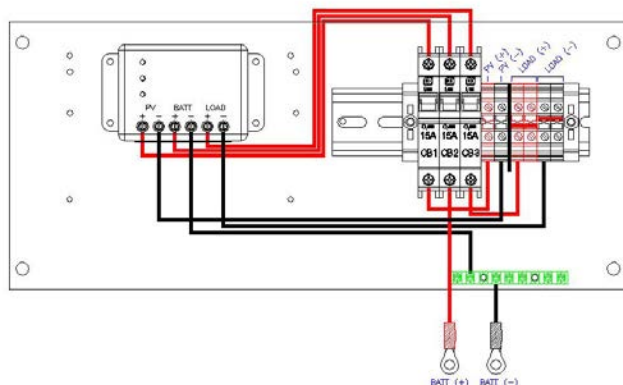
PRE Control Panel with a 10 amp ECO-N-T
