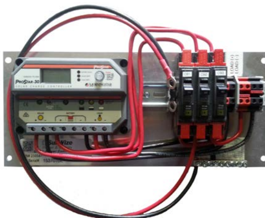
PRE Control Panel with a 30 amp ProStar
